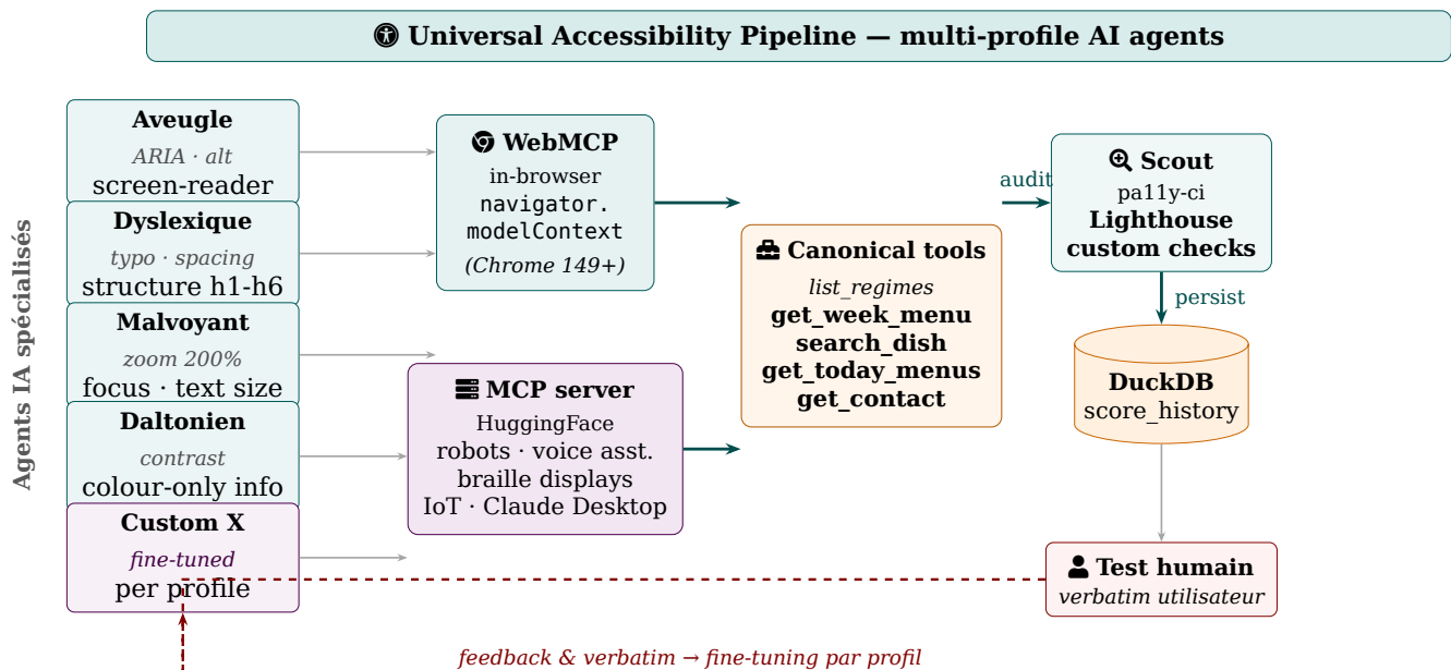
Figure 7: Universal Accessibility Pipeline: each AI agent simulates a specific WCAG profile and consumes the same canonical tools through either WebMCP (in-browser) or the MCP server (robots, voice assistants, braille displays, IoT). Scout audits the responses against multi-criterion rules; human verbatim closes the loop by fine-tuning each agent profile.
