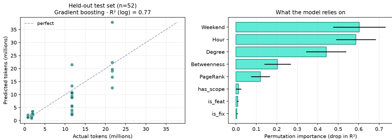
Figure 5: Left: predicted vs. actual token cost on the held-out test set — points hug the diagonal. Right: permutation importance (drop in test R^2 when a feature is shuffled). The model leans on timing and graph centrality , barely on commit type.
