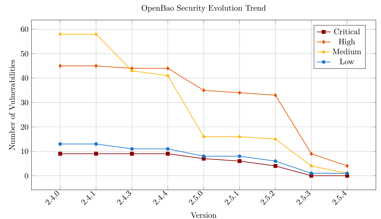
Figure 1: Security Improvement Trend: v2.4.0 to v2.5.4
