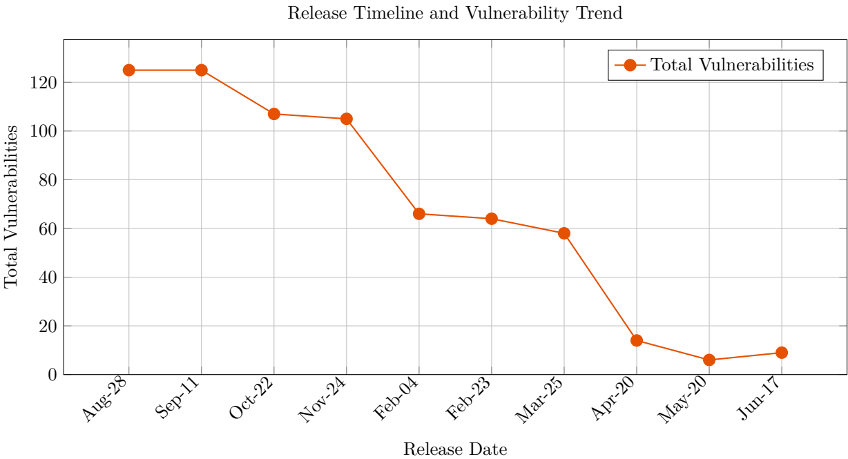
Figure 3: Release frequency and vulnerability reduction over time
