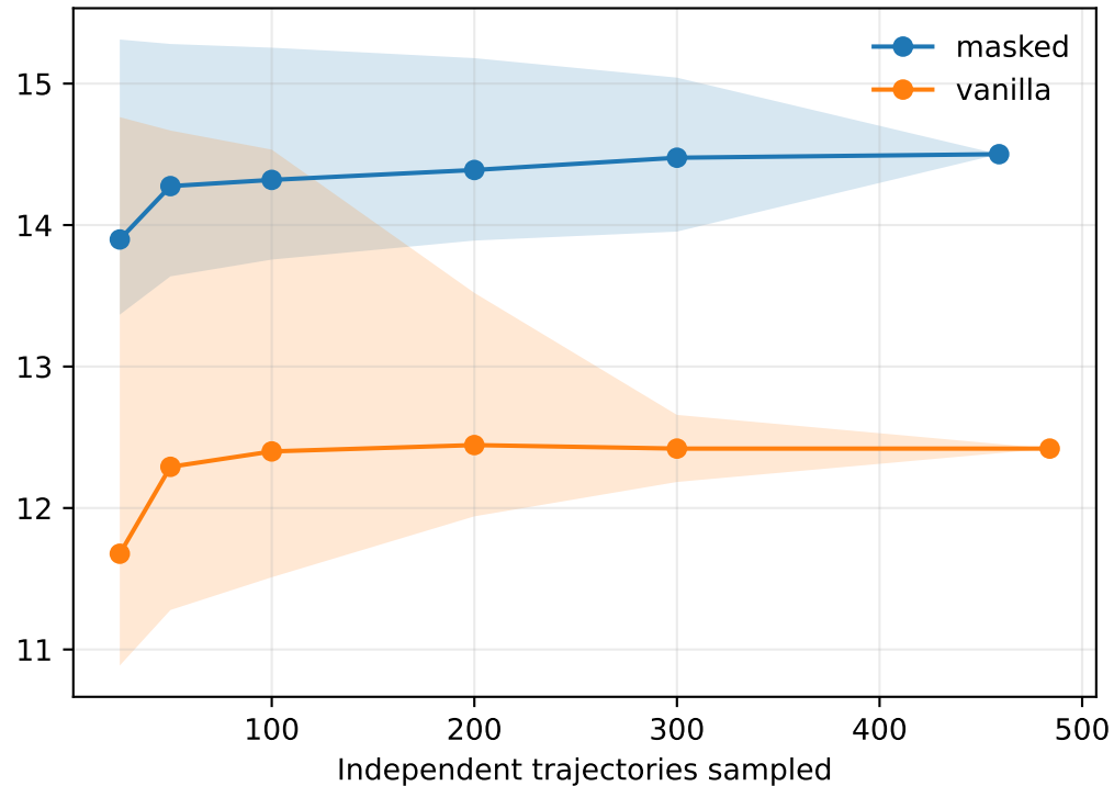
L403A q99 maximum E423-N179
