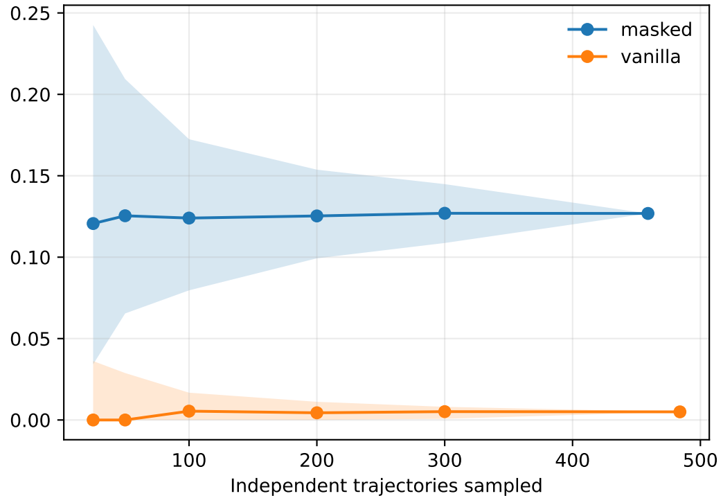
L403A any-shifted fraction
