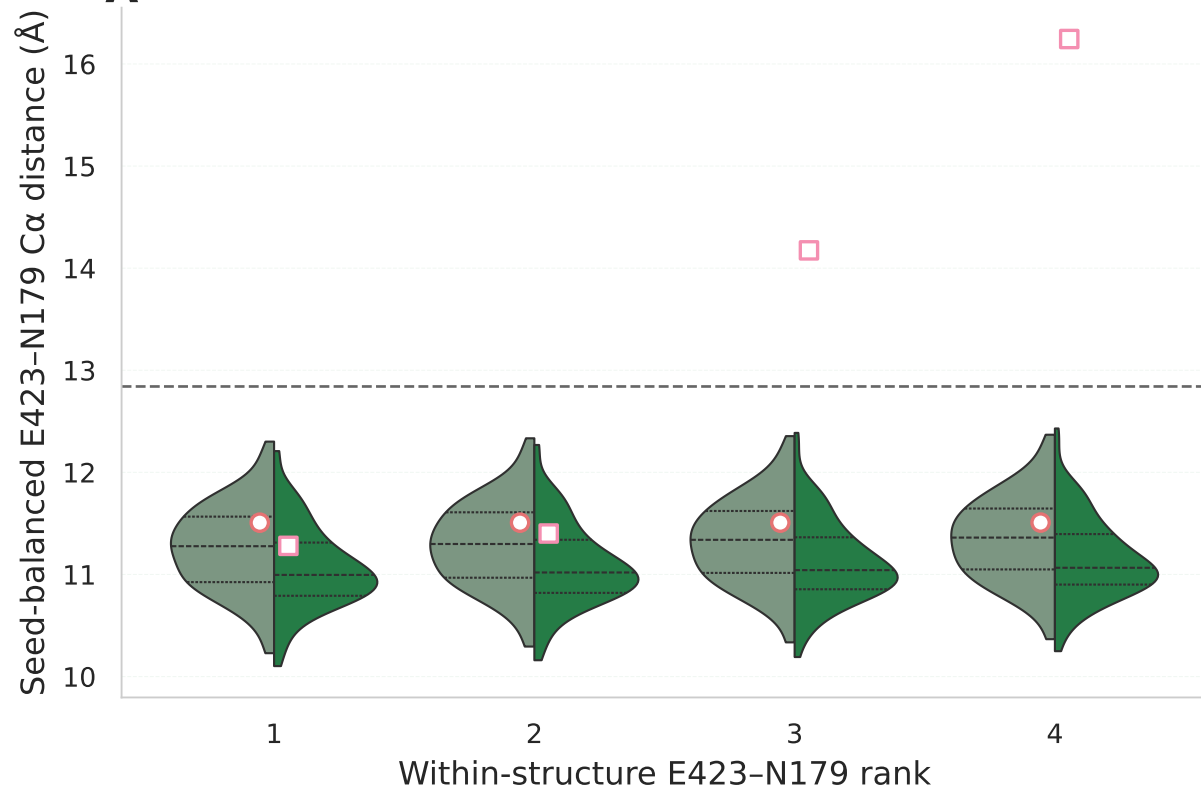
A Masked ensembles: ranked subunit distances
