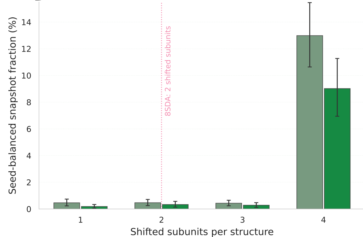
D Composition of the masked shifted tail
