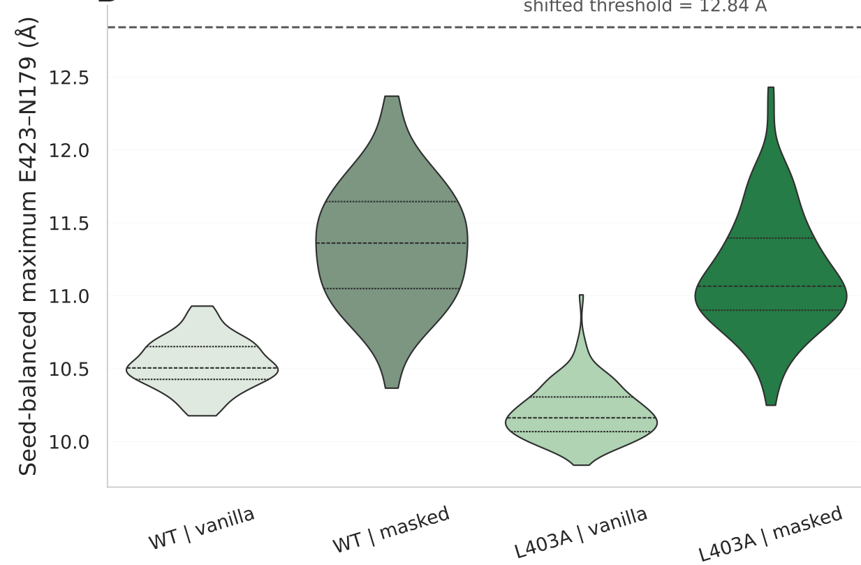
B Maximum tetramer distance
