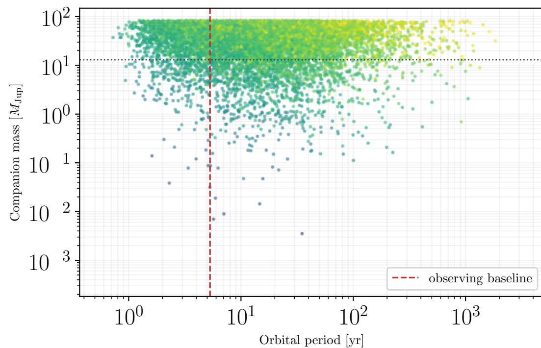
One planet: SNR-filtered
