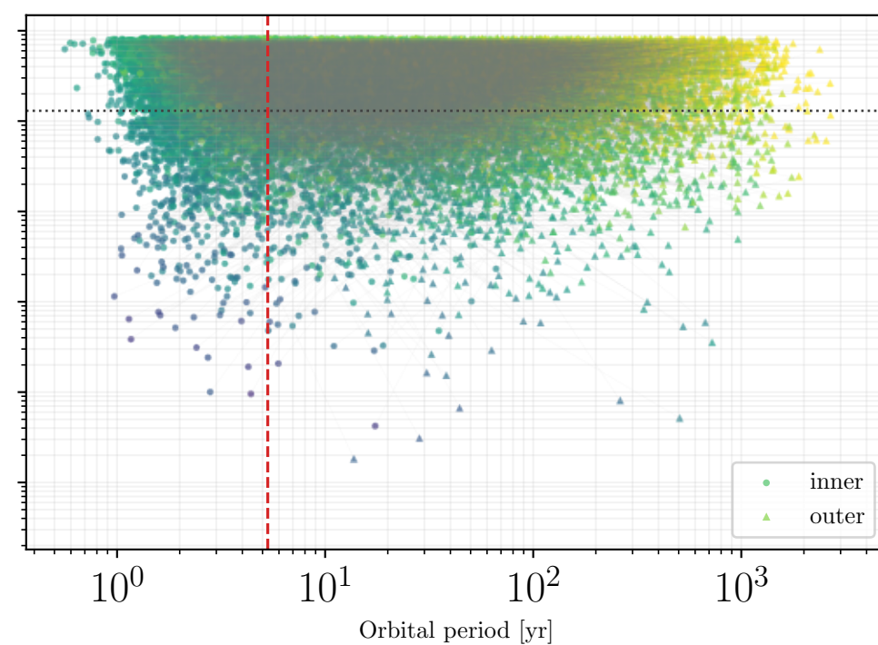
Two planets: SNR-filtered
