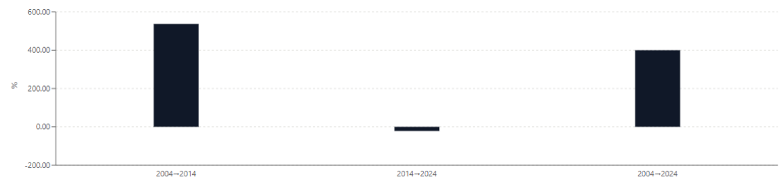
India annual-flow change by interval %
