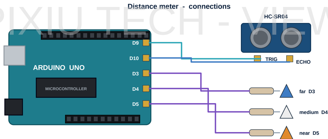
Figure 3.2 - Two wires for the sensor, three for the indicator lamps
