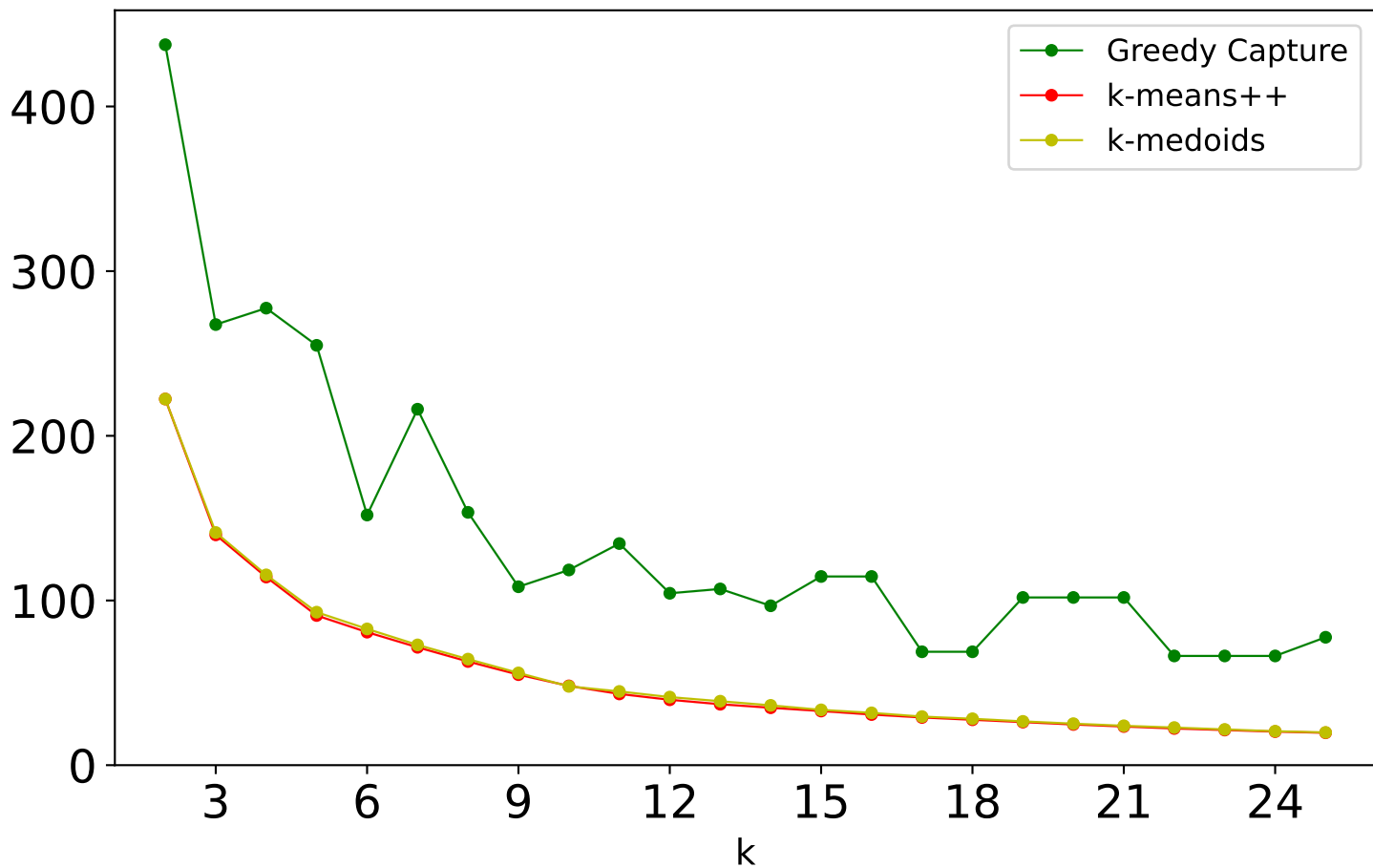
k-means Objective
