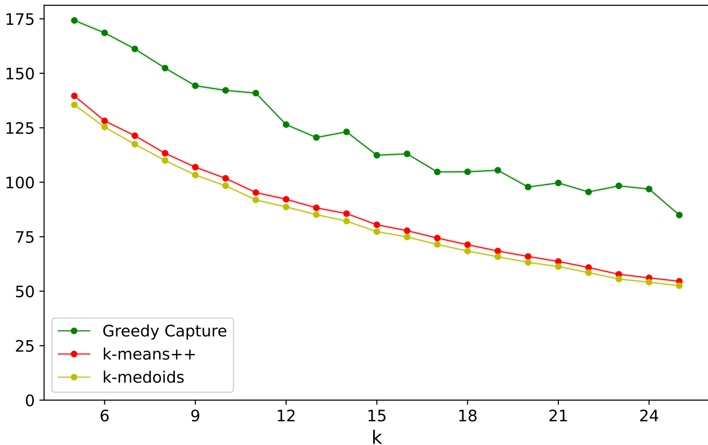
k-medoids Objective
