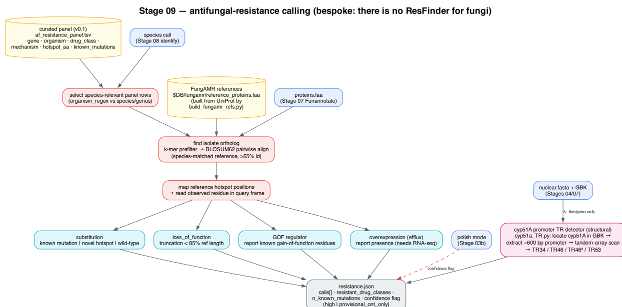
Figure 3: Stage 09 antifungal-resistance calling flow: species-relevant panel rows drive ortholog detection against species-matched FungAMR references; observed residues at panel hotspots are classified by mechanism; the cyp51A promoter TR detector runs structurally for A. fumigatus ; the polish mode sets the confidence flag.
