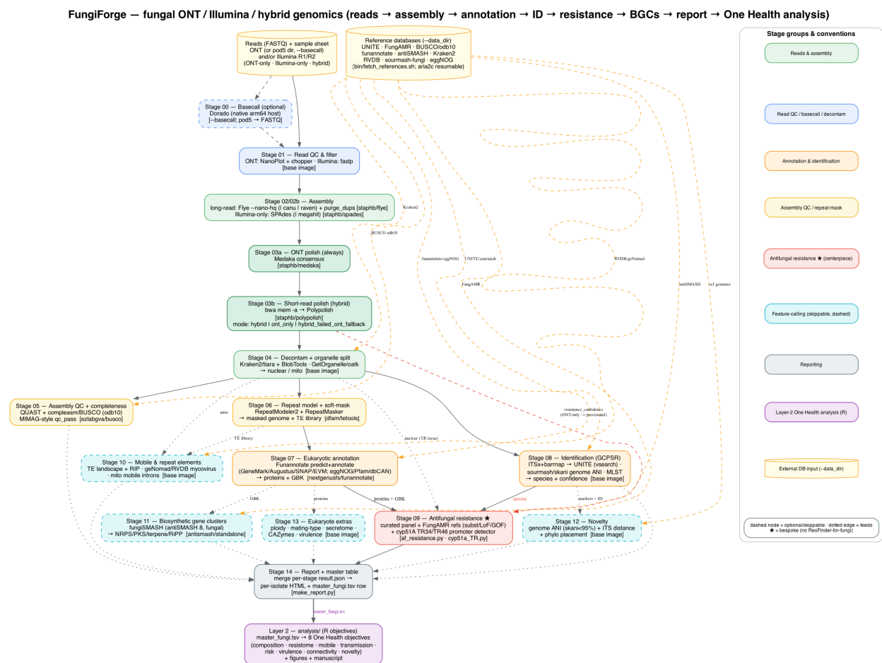
Figure 1: FungiForge Layer-1 pipeline DAG — the 15 stages colour-coded by group; the optional Dorado basecall and the four skippable feature-calling stages are dashed; external reference databases (amber) feed the ID/resistance/BGC/novelty stages; the antifungal-resistance stage (red, ★) is the bespoke centerpiece; everything converges on Stage 14, which emits master_fungi.tsv — the handoff to the Layer-2 One Health analysis.
