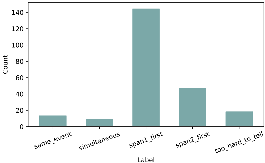
Temporal Order
