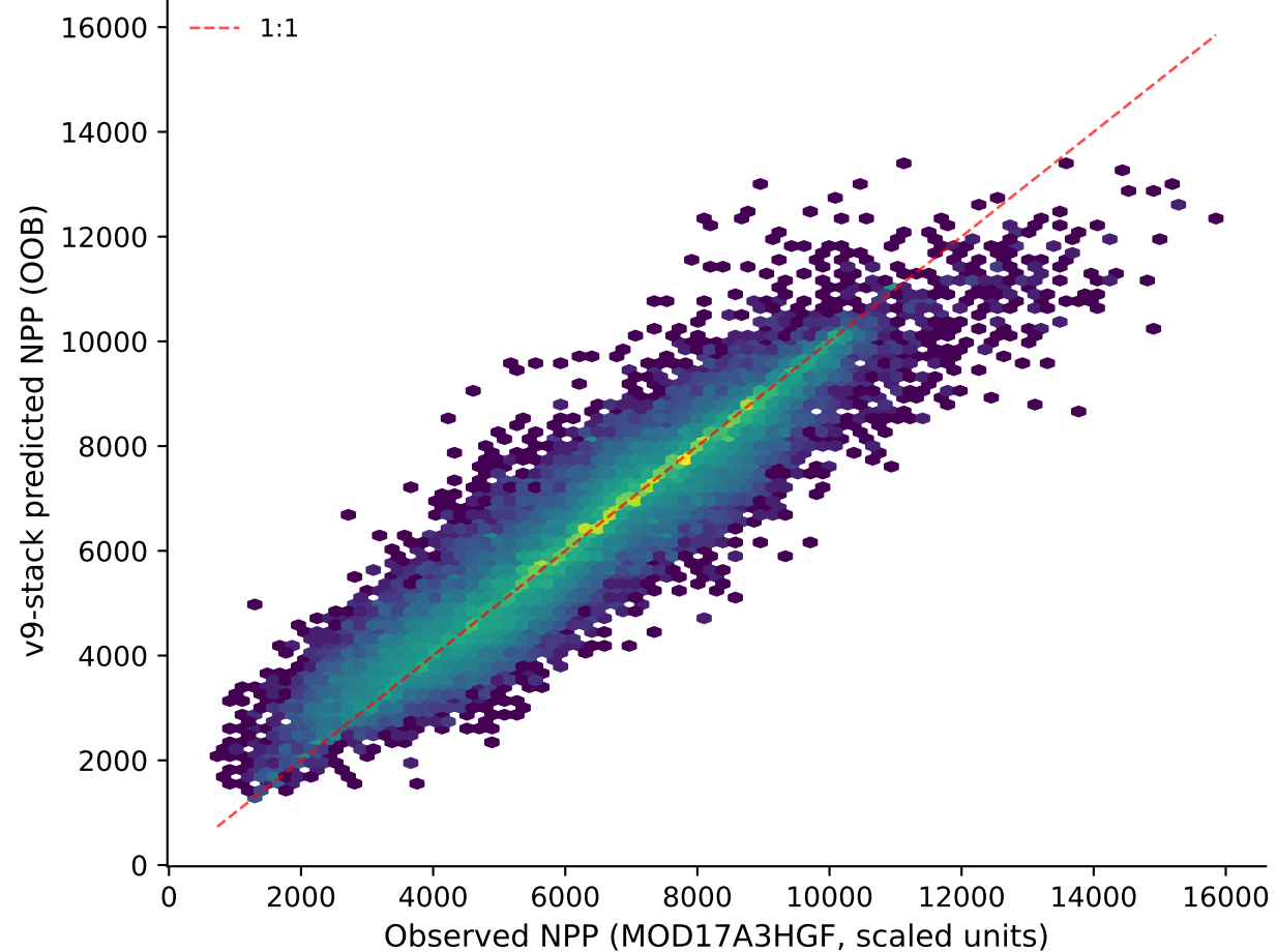
A. Predicted vs observed NPP OOB R^2 = 0.919 , RMSE = 509
