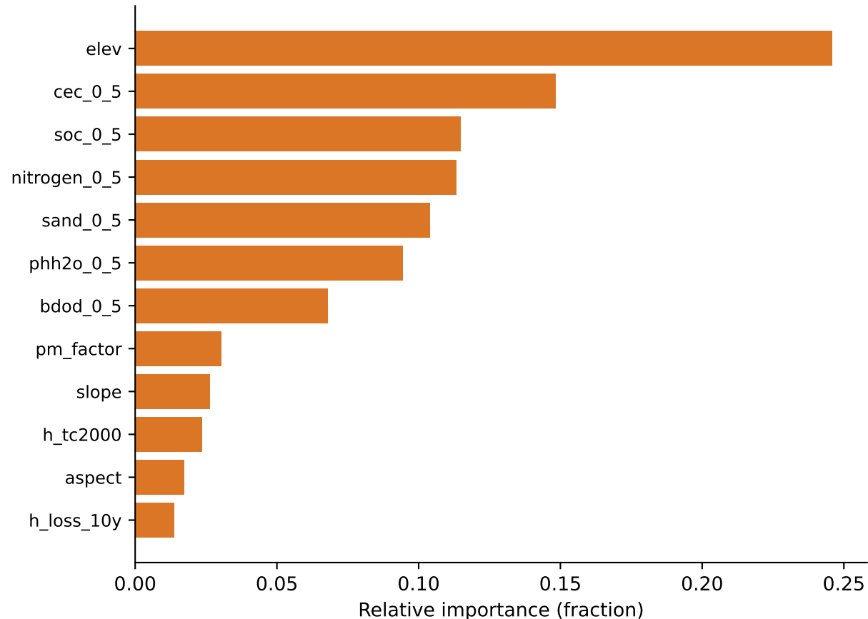
B. FIA-target: Asym v9 (biomass carrying capacity)
