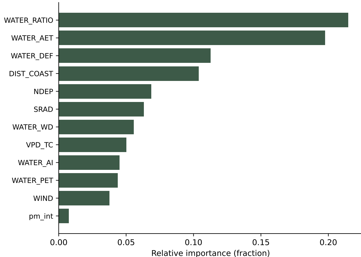
A. RS-target: MOD17 NPP (satellite observed)
