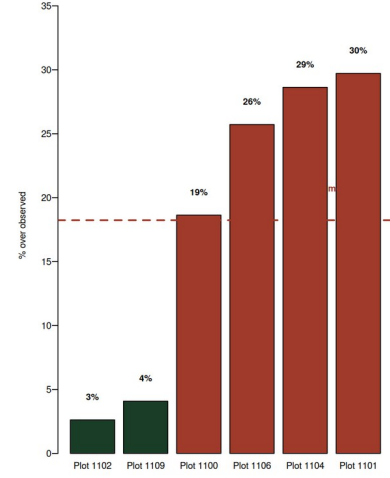
AGM long-horizon bias mechanism: under-mortality on disturbed plots + over-growth on slow plots TPA change over 10 years (%)
