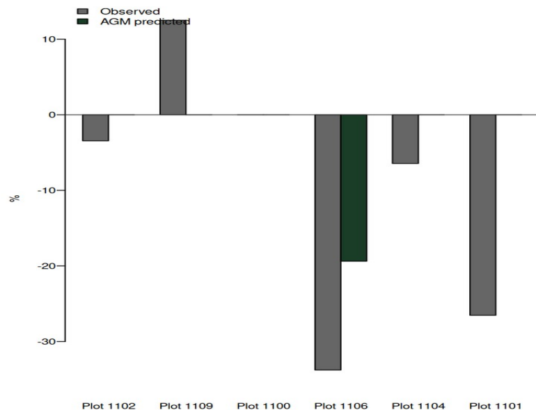
AGM long-horizon bias mechanism: under-mortality on disturbed plots + over-growth on slow plots
