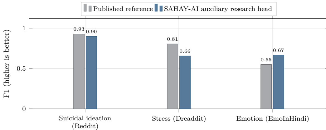
Figure 6: Auxiliary research heads against published references on the same datasets. These are not SAHAY safety metrics: they are diagnostics of what the adapted encoder represents, trained with capped data, and the EmoInHindi published bar is indicative only because that paper reports Hamming loss and Jaccard index rather than a comparable F1.
