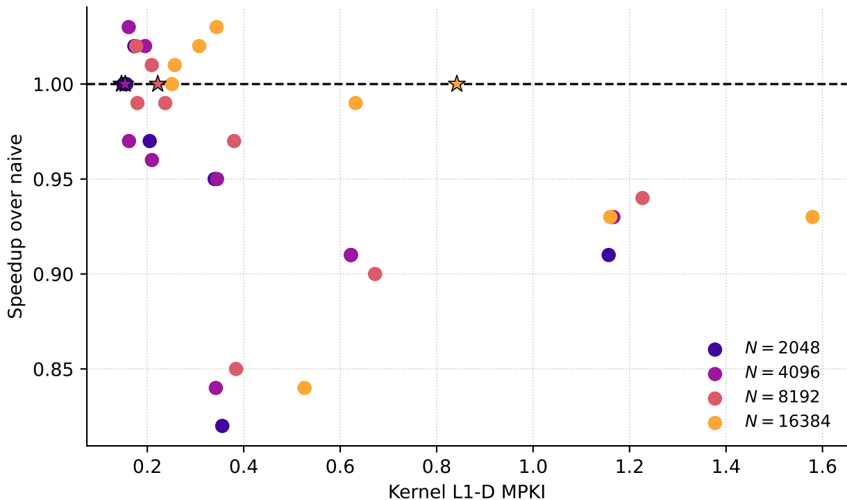
Lower MPKI does not translate into less time (stars = naive baseline)
