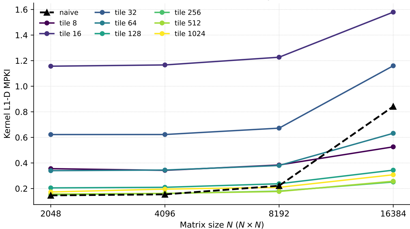
L1-D MPKI vs. matrix size, by tile size
