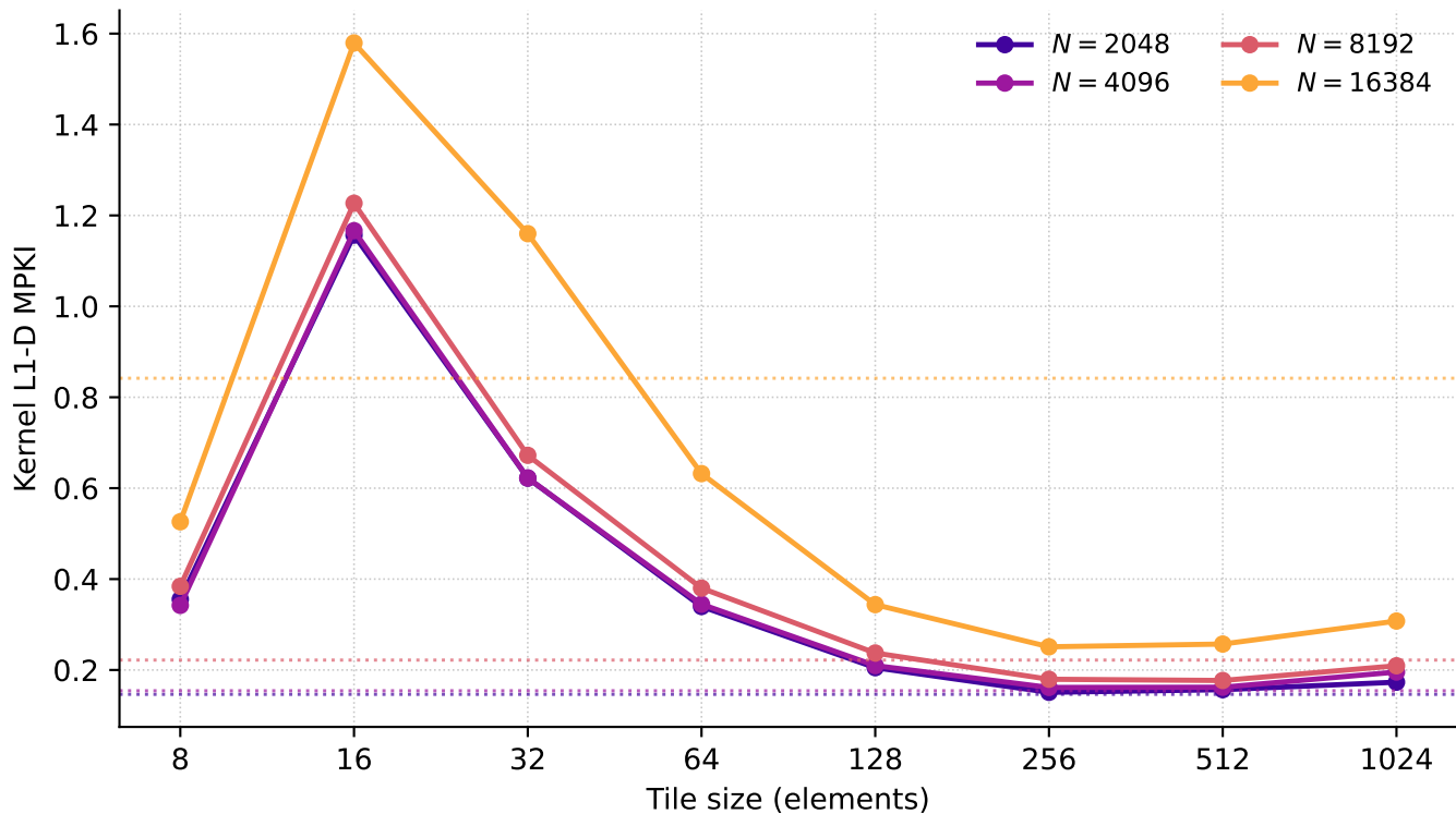
MPKI vs. tile size (dotted = naive baseline for that N )
