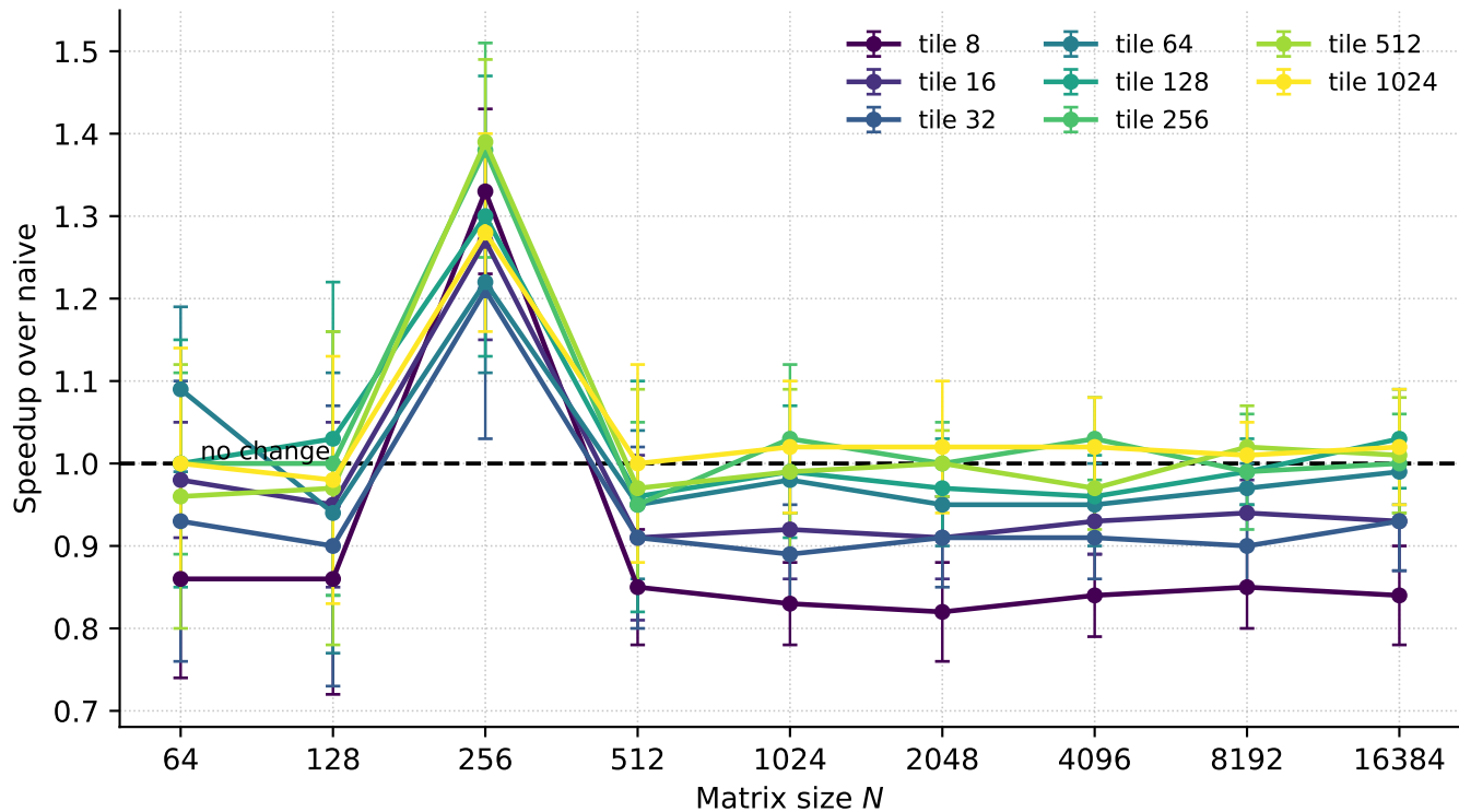
Speedup vs. matrix size, by tile size (error bars: \pm 1\sigma )
