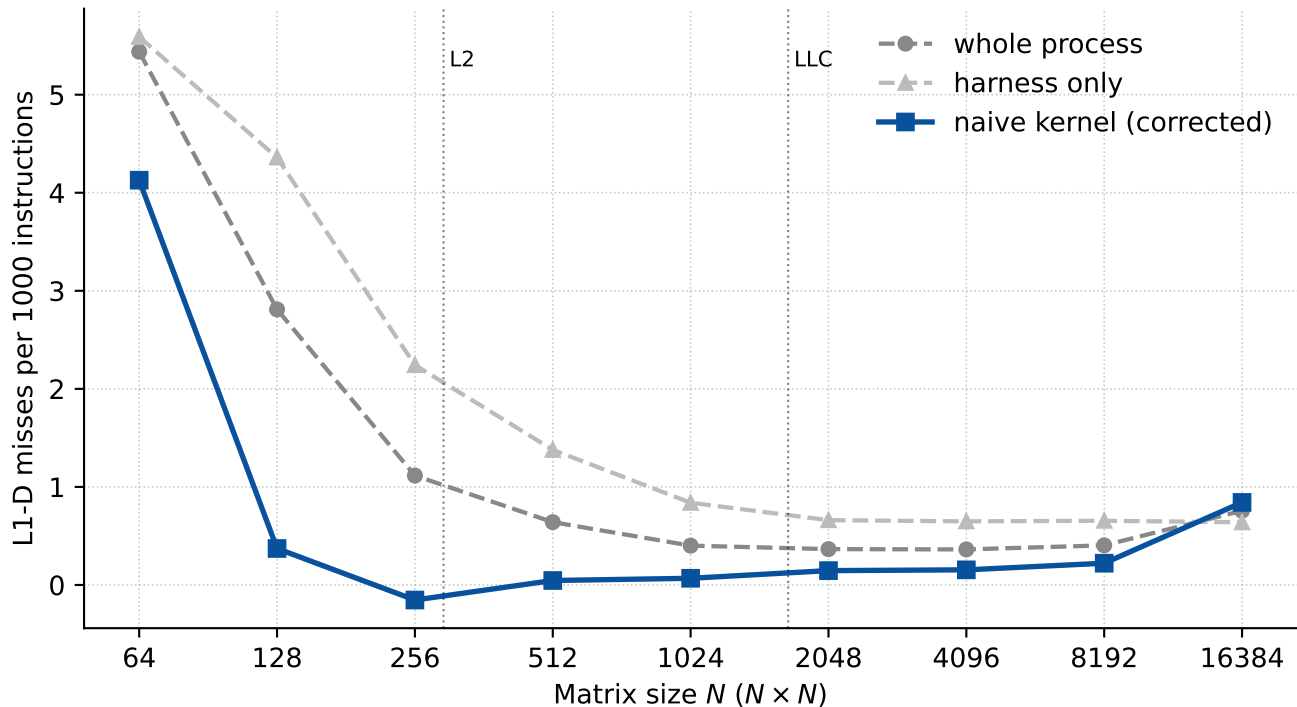
Baseline (naive) L1 data-cache MPKI
