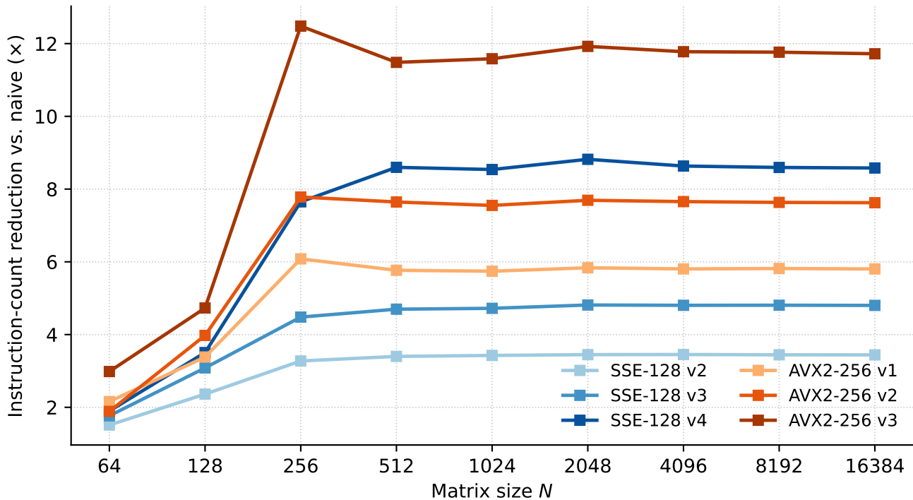
Retired-instruction reduction (kernel only)
