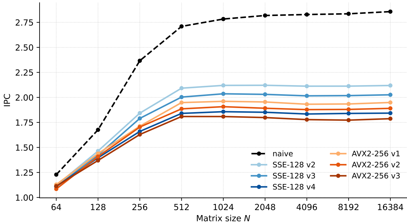
Instructions per cycle: fewer, denser instructions
