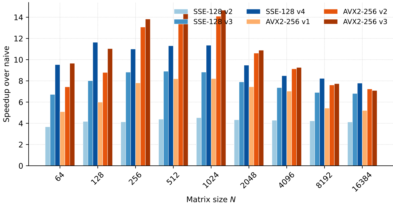
Speedup by SIMD width and matrix size
