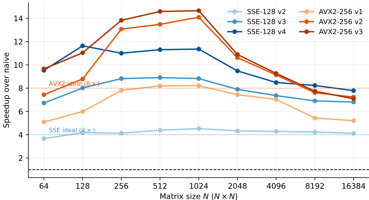
SIMD speedup vs. matrix size ( 3 \times 3 kernel)
