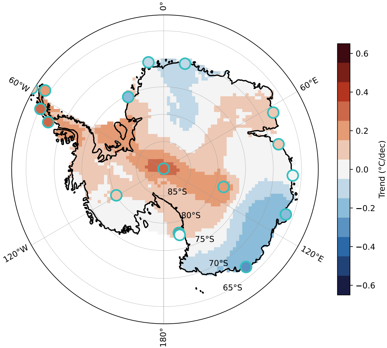
Temperature trends Bromwich et al. 1980-2020
