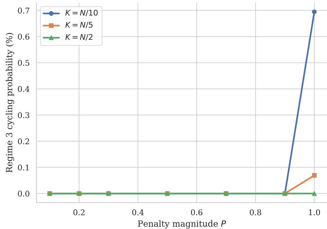
Kinship immunity scaling at \gamma_{stub} = 0.5
