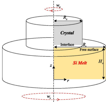
Axisymmetric melt domain in (r, z)
