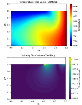
Reference T and |\mathbf{u}| (normalised, COMSOL)
