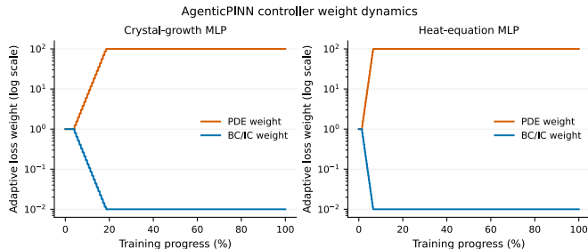
AgenticPINN loss weights during training (log scale)
