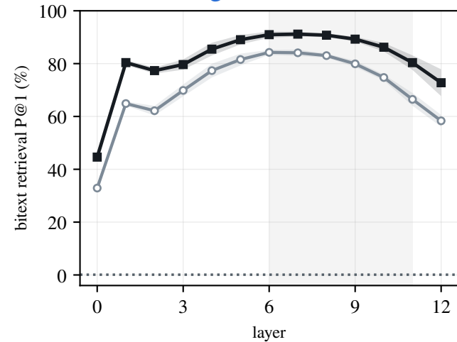
English–Dutch
