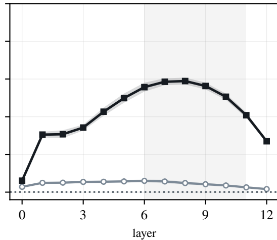
Dutch–Chinese
