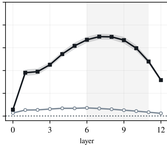
English–Chinese
