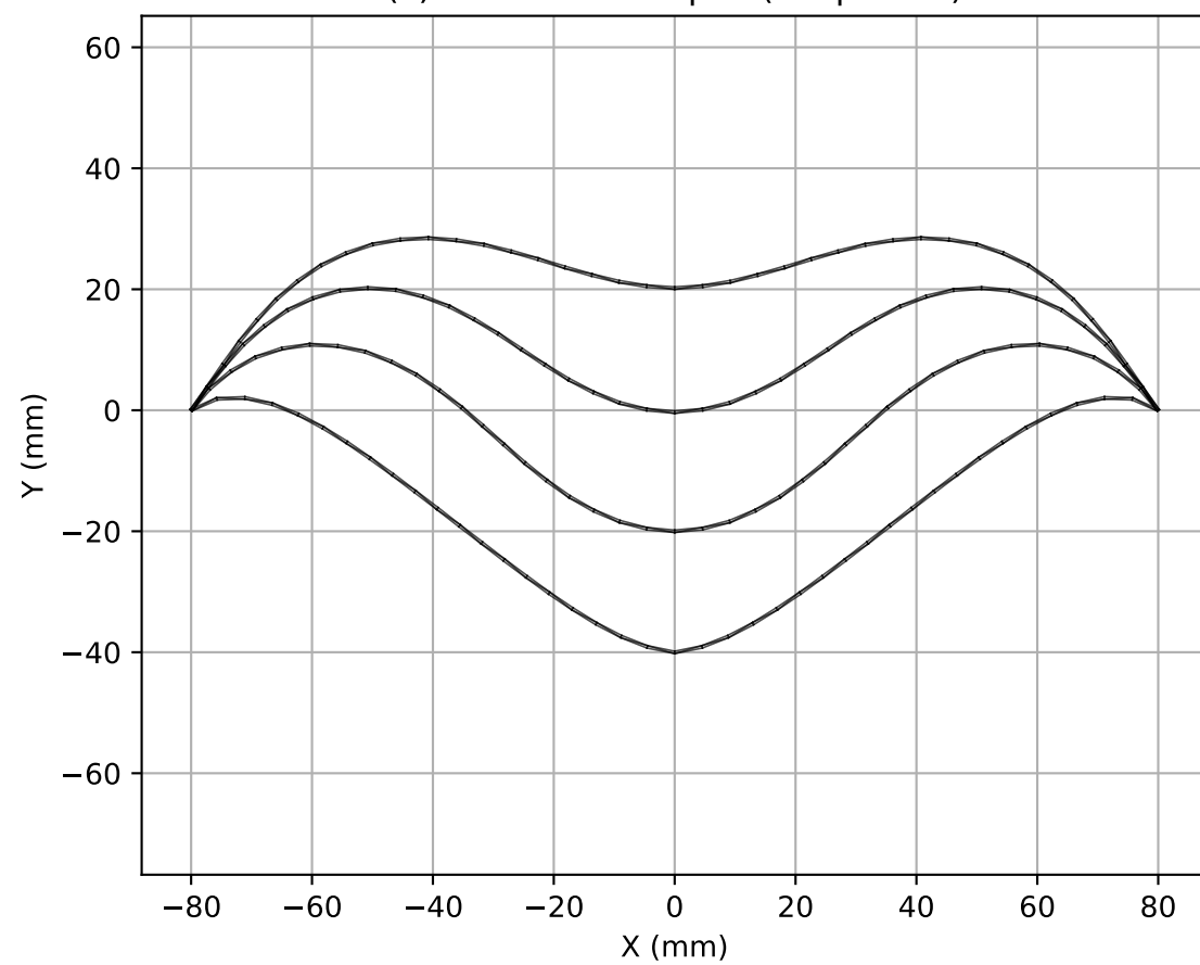
(c) Deformed shapes (snapshots)
