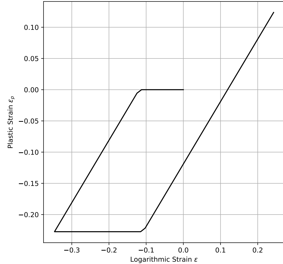
Plastic Strain \epsilon_p vs Log Strain \epsilon
