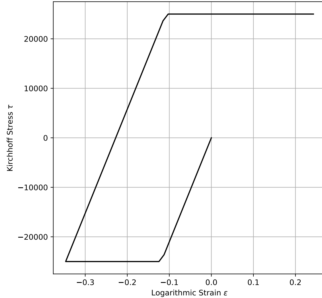
Kirchhoff Stress \tau vs Log Strain \epsilon
