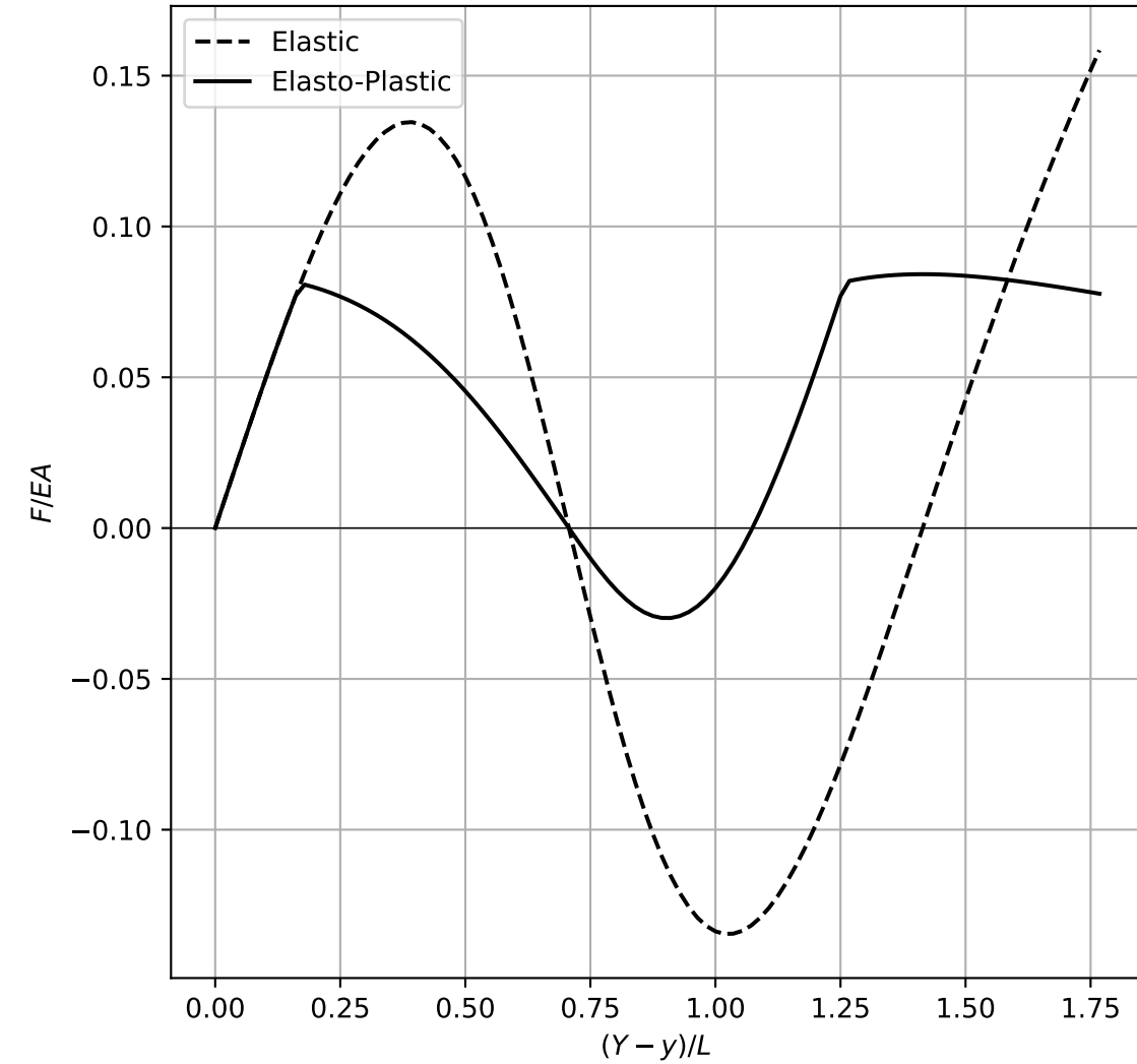
Load-Displacement Path
