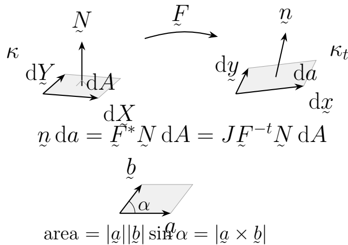
Figure 2.9: Deformation of oriented surface measure.
