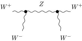
\FourPointCorr half-box
