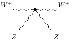
\FourPointCorr flat-contact
