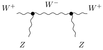
W/Z half-box
