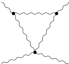
\FourPointCorr dispatch
