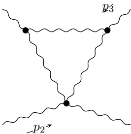
Selected momenta
