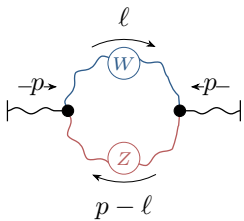
two circ ewbosons
