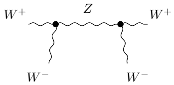
\FourPointCorr half-box
