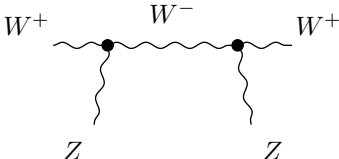
W/Z half-box
