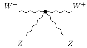
\FourPointCorr flat-contact
