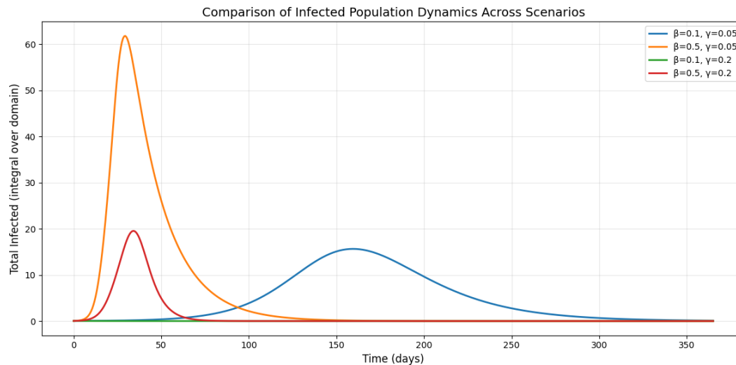
Figure 2: Comparison of Infected Population Dynamics Across Scenarios
