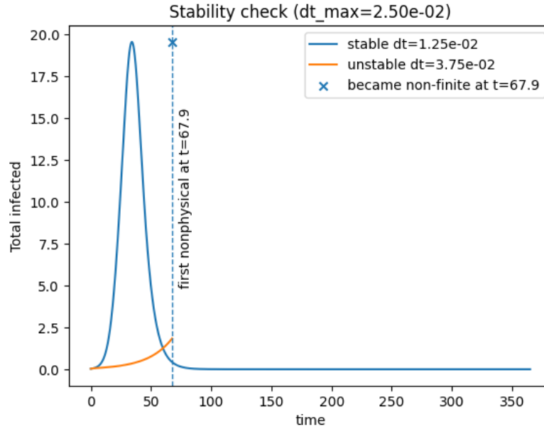
Figure 1: Stability investigation by increasing the time step
