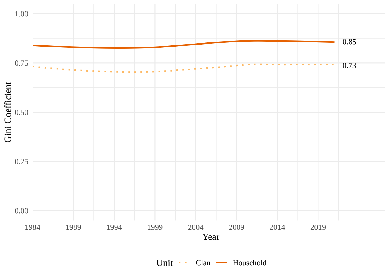
Figure 3B: Wealth inequality from 1984 to 2021
