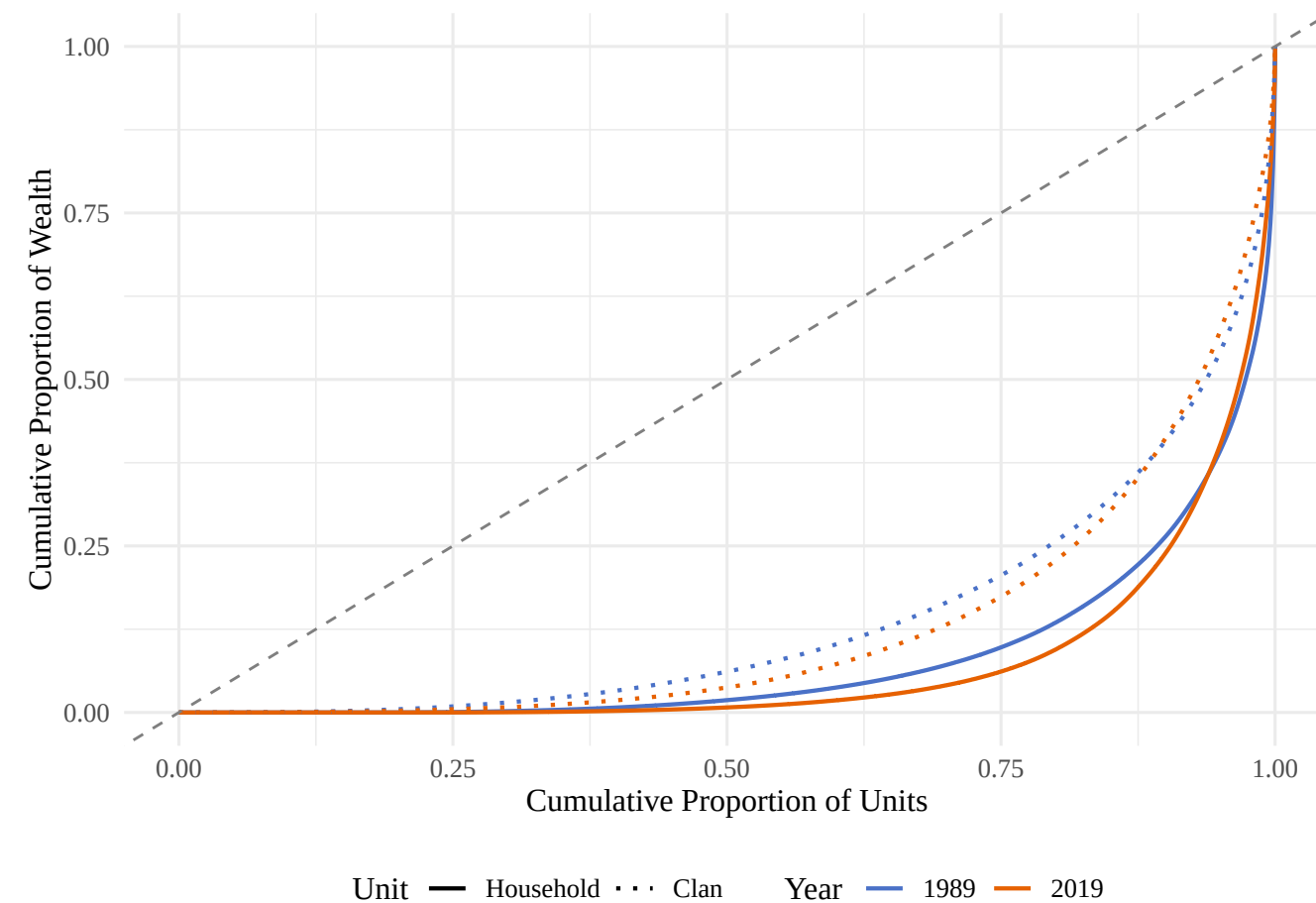
Figure 3C: Distribution of wealth in 1989 and 2019
