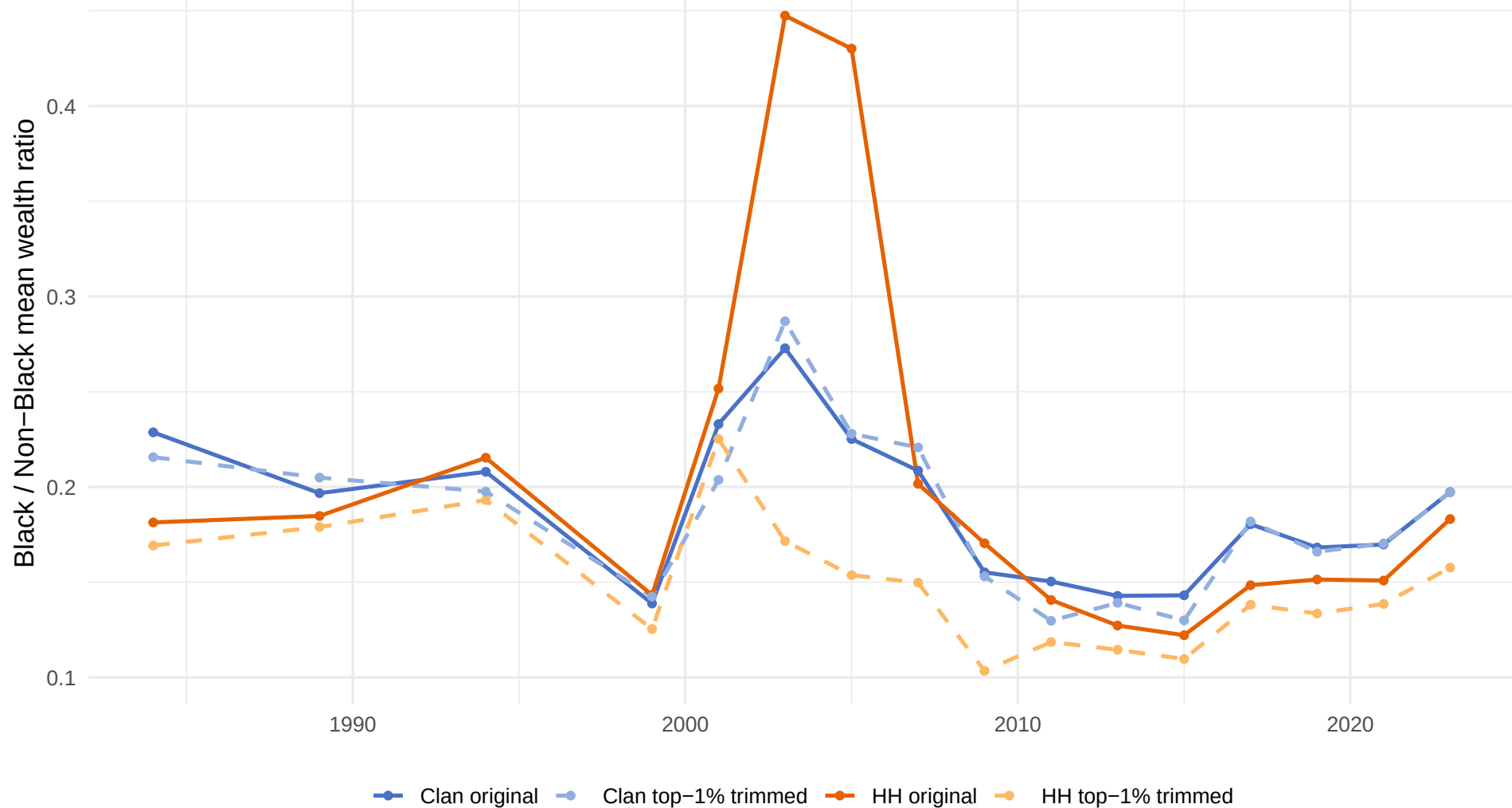
Diagnostic 2: Wealth ratio original vs. top-1% weight-trimmed
