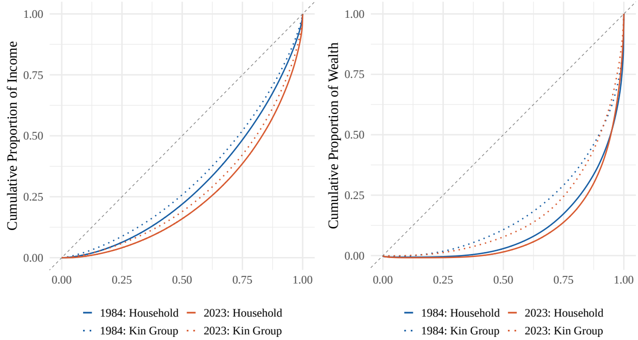
Figure 2. Lorenz Curves at the Household and Kin Group Levels
