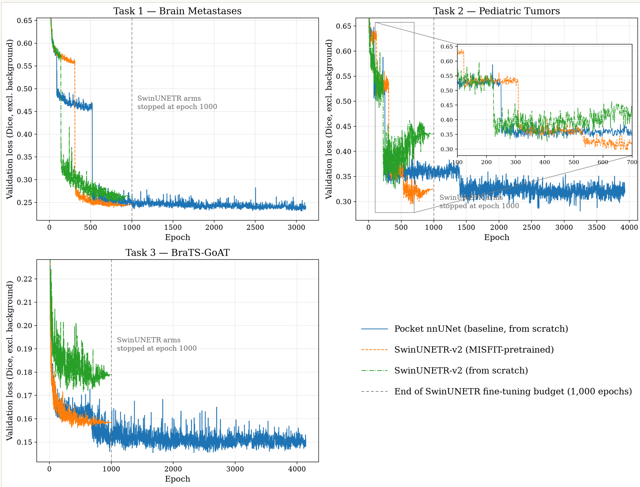
Figure 1. Validation loss (Dice, excl. background) across training. The MISFIT-pretrained arm reaches within 3.5–7.3% of the baseline’s fully converged floor inside its 1,000-epoch budget — in far fewer epochs than the baseline needs (means: 3,107 / 3,908 / 4,252). The from-scratch SwinUNETR fails to converge at all on Task 2.
