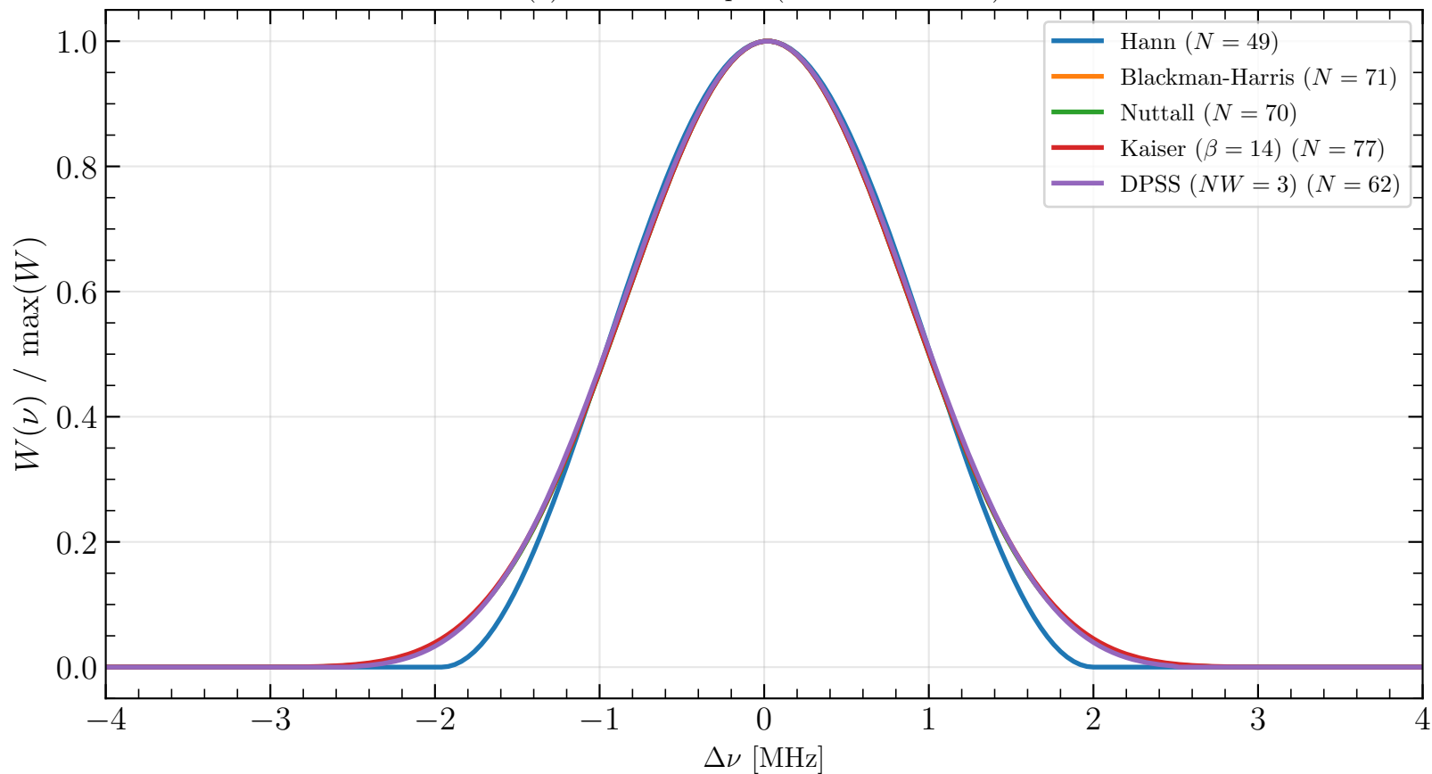
(b) Transfer Function (Sidelobe Suppression)
