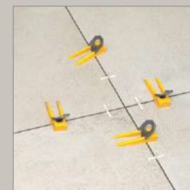
After Lavelling Process Leave Int For 8-10 Hrs.
