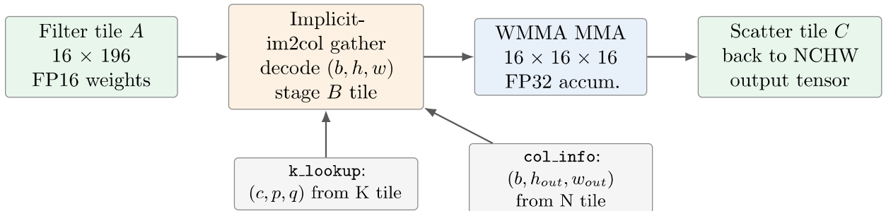
Figure 3: Conv2 fused implicit-GEMM mapping. The kernel avoids materializing the full im2col matrix by decoding each output-column coordinate and staging only the WMMA tile needed for the current warp.
