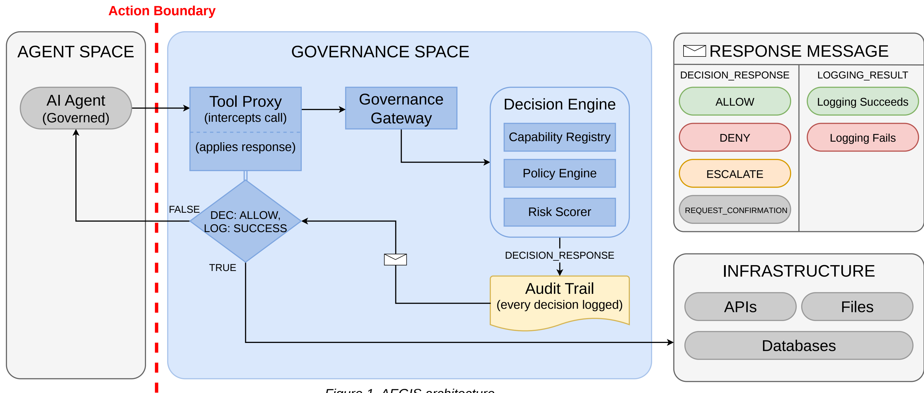
Figure 1. AEGIS architecture
