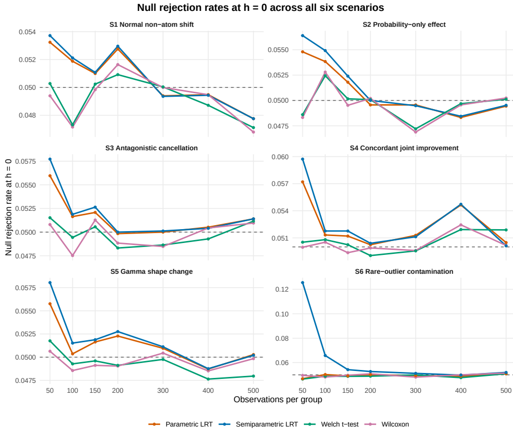
Figure 6: Null rejection rates at effect level h = 0 across all six simulation scenarios. The dashed line marks 0.05.
