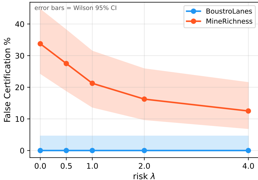
FC rate vs. risk \lambda
