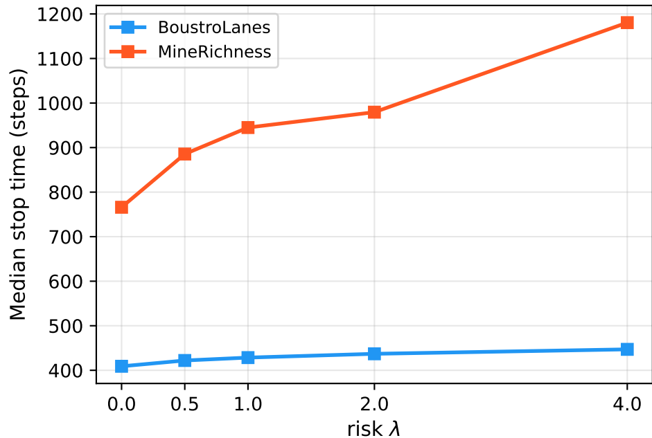
Median stop time vs. risk \lambda
