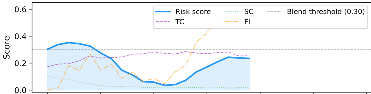
MineRichness (seed=42)
