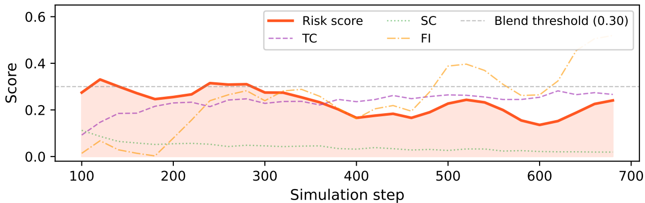
MineRichness (seed=42)
