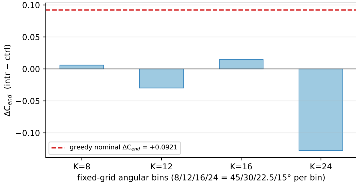
Bin-sensitivity of the configuration counter
